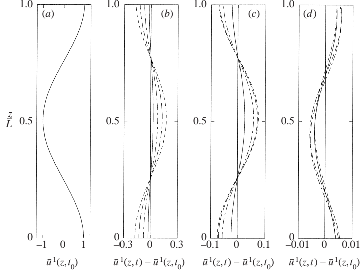
FIGURE 9. Evolution of the fundamental mode \bar{u}^1 of the mean flow profile in Simulations ANS, AMS and ASS. Here the velocity scale is U_0 , the amplitude of the perturbation imposed at t = t_0 . (a) Profile of \bar{u}^1 at t = t_0 . (b, c, d) Profile of the fundamental profile increment \bar{u}^1(z, t) - \bar{u}^1(z, t_0) at t = t_0 (solid line), t = t_0 + \tau_0 (dot-dashed curve), t = t_0 + 2\tau_0 (long-dashed curve), t = t_0 + 3\tau_0 (dashed curve) and t = t_0 + 4\tau_0 (dotted curve) in Simulations (b) ANS, (c) AMS and (d) ASS.
